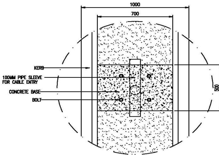
PLAN VIEW (FOR CONCRETE BASE) APPENDIX B.2
