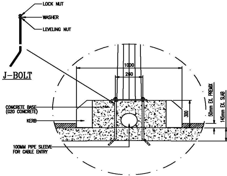
SIDE VIEW (FOR CONCRETE BASE) APPENDIX B.1
